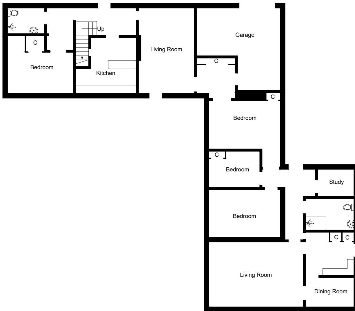
Ground Floor
